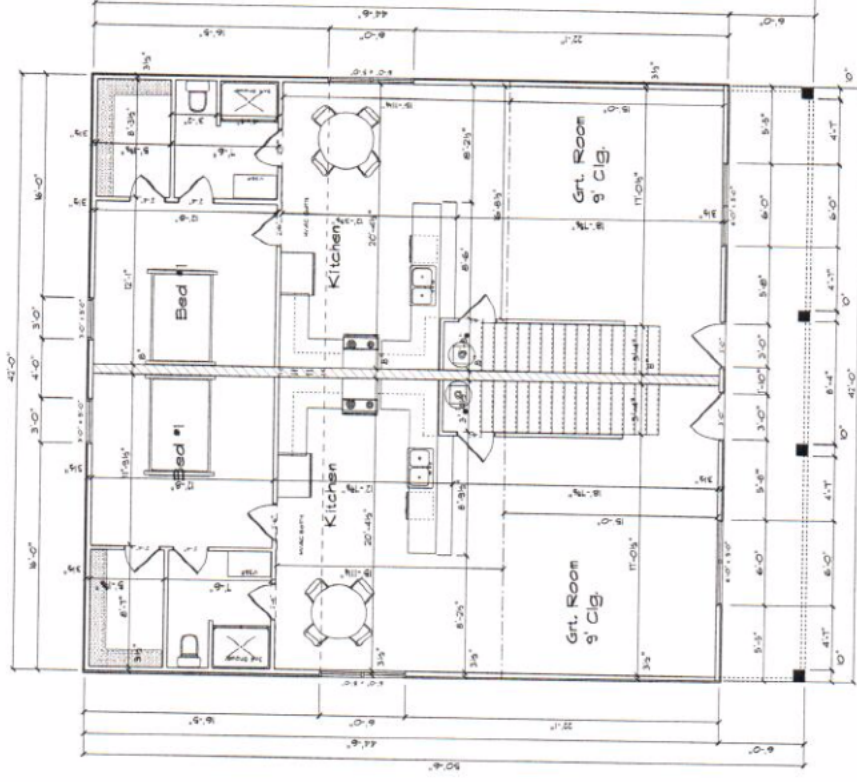
MAIN FLOOR PLAN SCALE 1/4" = 1'-0"
